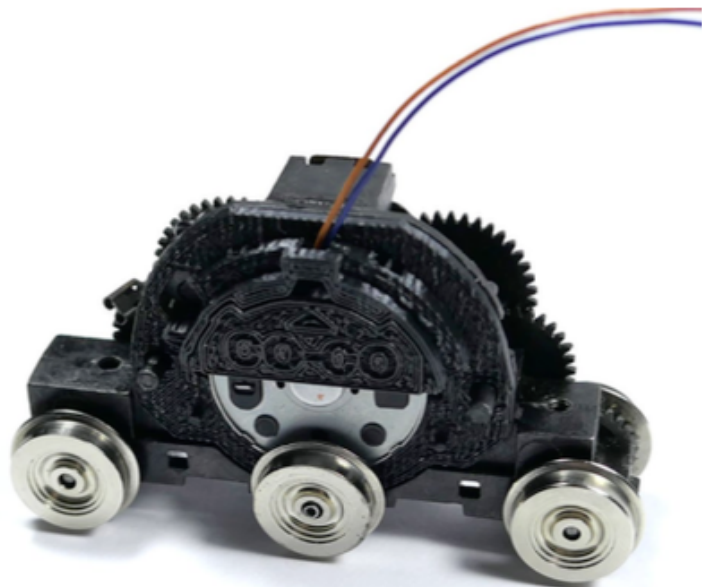
HA1 (6V) motor adaptor in a Hornby Class 37 bogie
